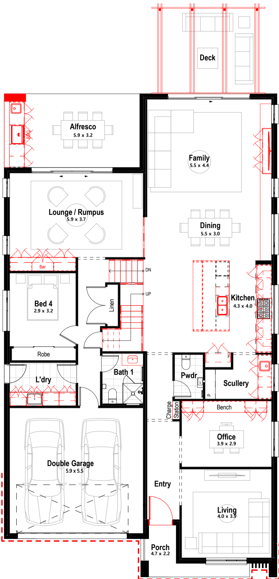
GROUND FLOOR
